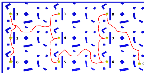
Fig. 5. Path produced by the Multi-T-RRT enhanced with useful-cycle addition on the Stones problem, for a running time of 5 s. The labels show the order in which the waypoints are visited.
