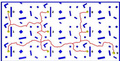
Fig. 3. Path computed by the Multi-T-RRT on the Stones problem, going through all ten waypoints. The cost is the inverse of the distance between the 2-DoF yellow disk and the blue rectangular-shaped obstacles.
