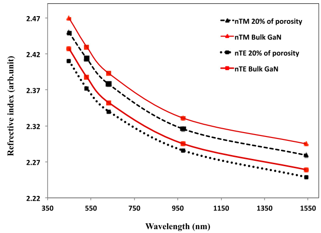
FIG. 5. Ordinary and extraordinary refractive indices dispersion for bulk and porous (20%) GaN samples.
