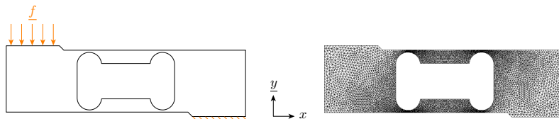
Figure 1: Weight sensor model problem (left) and associated finite element mesh (right).
