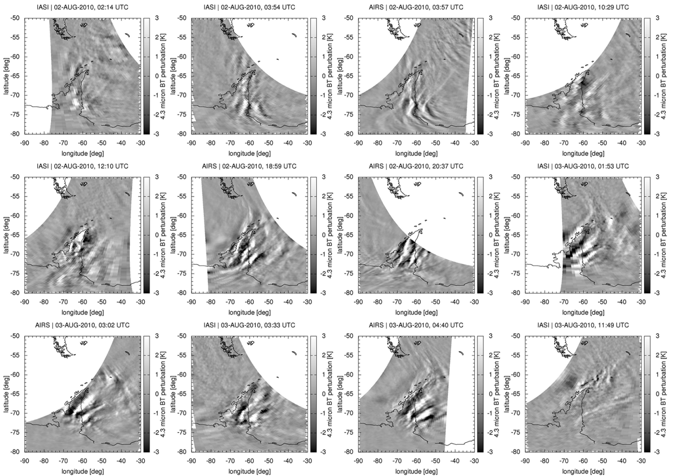
Figure 7. 4.3 \mu\text{m} brightness temperature perturbations showing stratospheric temperature perturbations of a mountain wave event at the Antarctic Peninsula on 2–3 August 2010. Plots show observations from selected AIRS and IASI overpasses in temporal order.
