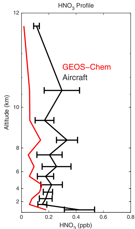
Figure 4. Average HNO 3 profiles from aircraft campaigns (PEM-West B and PEM-Tropics A) and from GEOS-Chem sampled along the flight paths. Error bars indicate 1 standard error from the mean.
