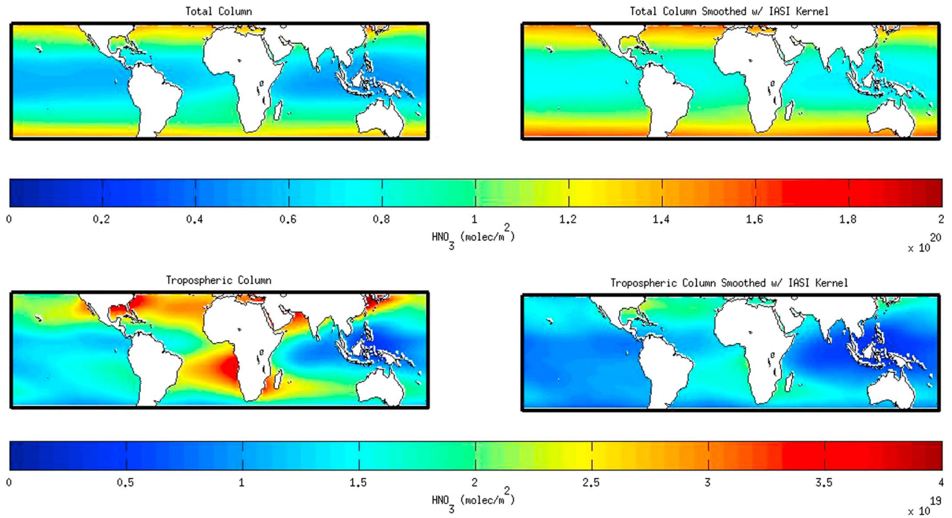
Figure 1. GEOS-Chem simulated HNO 3 columns. Subplots contain the (top) total column and total column after smoothing with IASI averaging kernels and (bottom) tropospheric column and tropospheric column after smoothing with IASI averaging kernels.
