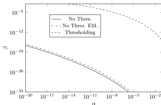
Figure 6.1: Authentication performance using model estimation with the EM algorithm ( N = 2000 , N_o = 2000 , \sigma = 52 , m_b = 50 , m_w = 150 ). The asymptotic expression is used to derive the error probabilities.
