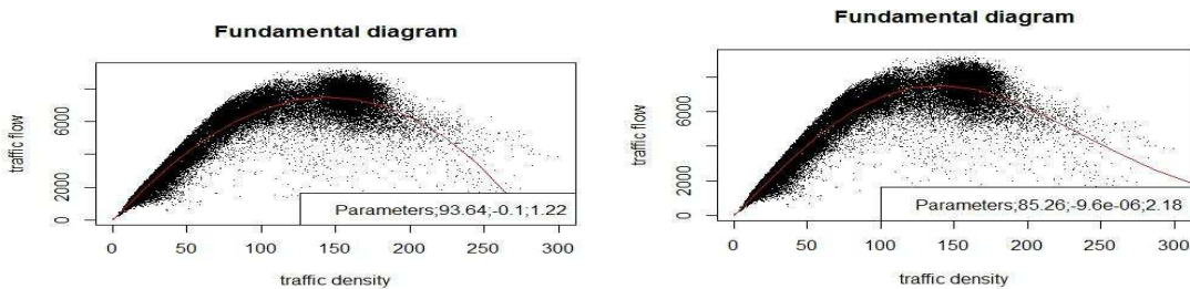
Figure 3. Global fundamental diagram in 2002 fitted with (a) a generalized power model (b) a generalized exponential model Number of data: 53677; Residual standard error for (a) : 707.4 ; for (b) : 696.5
