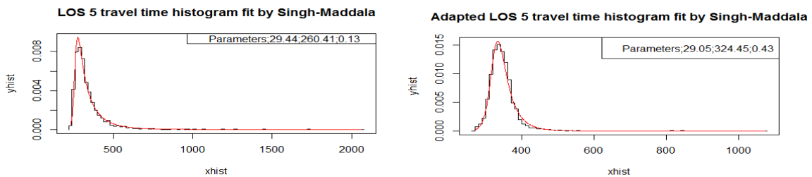
Figure 9. Histogram of original and adapted LOS 5 travel times fit by Singh-Maddala distribution in 2002
