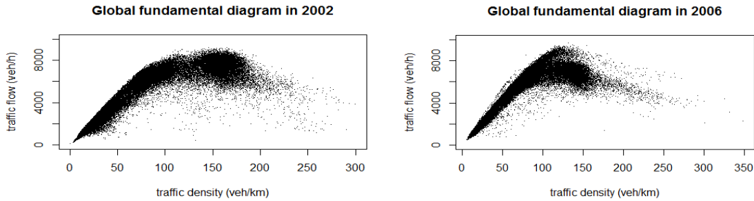
Figure 2 (a) Global fundamental diagram in 2002 (b) Global fundamental diagram in 2006 direction Paris to the East
