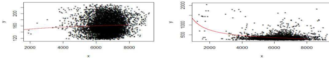
Figure 8. Non-linear regression between travel times (variable y) and flows (x) in 2002 for (a) LOS 3 (b) LOS 5
