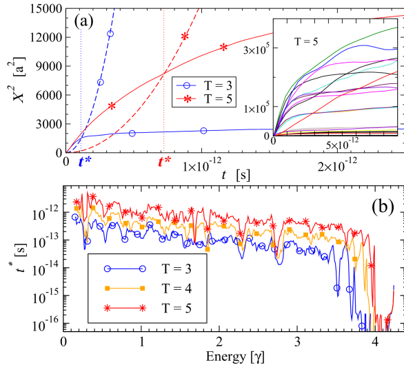
Fig. 2. (a) Average square spreading versus time t at E = 1.0 eV in perfect Penrose approximants T = 3 and 5: (dashed line) Boltzmann X_B^2 and (line) non-Boltzmann X_{\text{nB}}^2 (inset: X_{\text{nB}}^2 versus time t at different energies in approximant T = 5 ). (b) Time t^* in perfect Penrose approximants (see text).
