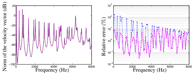
Fig. 7 FRF of the beam with holes: (Left figure) FE solution (—) and WFE-based interpolated solution (- - -); (Right figure) relative error of the WFE-based interpolated solution, with adaptive refinement (-●-) and without adaptive refinement (-●-).
