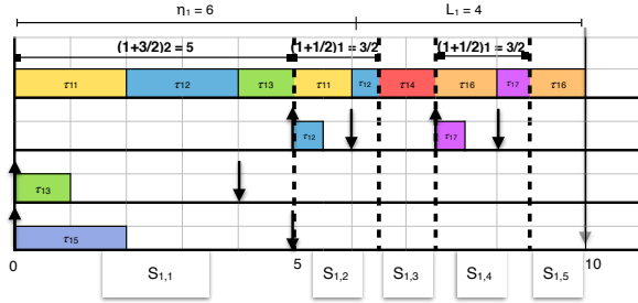
Figure 3: Example of stretching scheduling method for DAGs.
