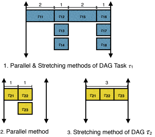
(a) Example 2: DAG set consists of two periodic implicit-deadline DAG tasks. (1) Both scheduling methods (parallel & stretching) of DAG \tau_1 . (2) The structure of DAG \tau_2 when the parallel scheduling method is used. (3) The structure of DAG \tau_2 when the stretching scheduling method is used.
