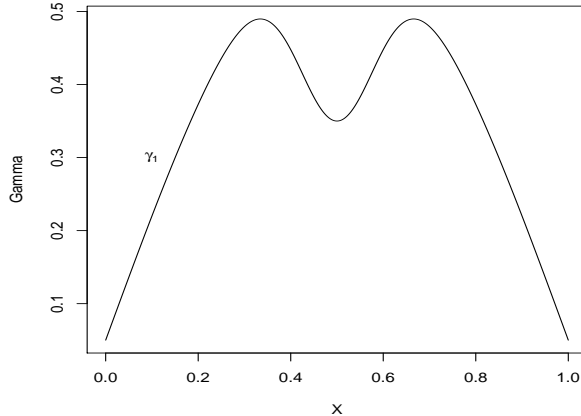
Figure 1: Pattern of \gamma_1(\cdot) on [0, 1] .
