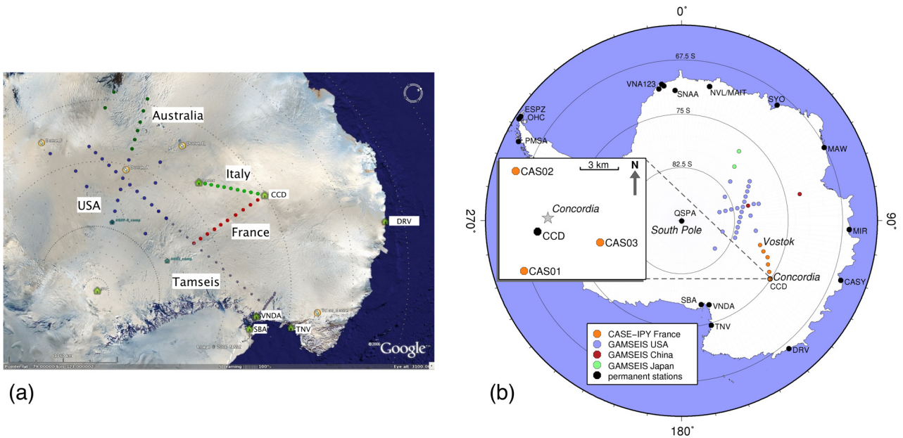
Figure 2. The East Antarctica IPY deployments. (a) As planned at the time of the submission of the funding application for the CASE-IPY experiment (February 2007). The earlier TAMSEIS deployment is also shown. (b) As deployed in the field at the time of the CASE-IPY deployment (2011).
