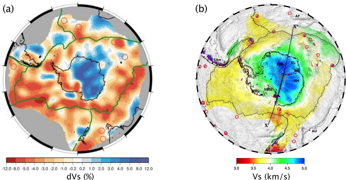
Figure 12. Surface wave tomographic maps of Antarctica at 100-km depth. (a) Results from permanent stations only (after Sieminski et al. [2003]). (b) Preliminary results using permanent and POLENET stations (after An et al. [2011]).
