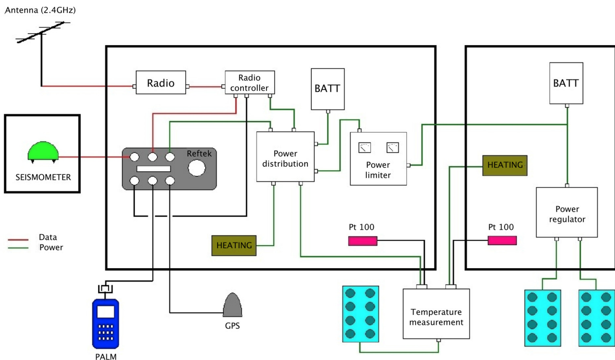
Figure 3. Design of the first prototypes of the CASE-IPY autonomous seismic stations (3-box design with radio transmission to Concordia base). Heating and radio transmission were removed, and the acquisition (Reftek box) and battery (BATT) boxes were merged for the final design.
