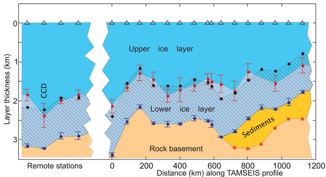
Figure 10. Two-layer ice structure in East Antarctica and Greenland from P-wave receiver functions (after Wittlinger and Farra [2012]). The hatched area has a constant thickness equal to the mean thickness of the lower layer. Remote stations (left) are from left to right: SUMG (Greenland), CCD (Concordia), QSPA (South Pole) and P061 (a Polenet station, see Figure 11a). Other stations are from the TAMSEIS experiment (N132-N020).
