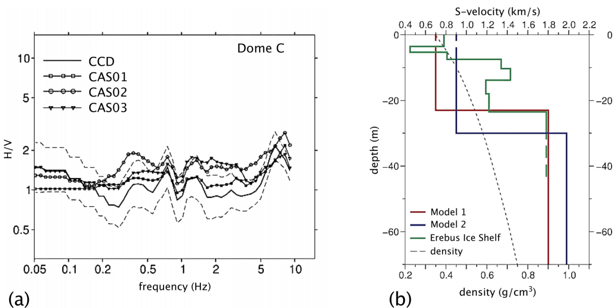
Figure 9. Snow structure at Dome C (after L  v  que et al. [2010]). (a) Mean spectral ratios of horizontal to vertical motion determined from noise at the four Dome C stations. The 1-sigma confidence level is similar for the different curves, and is shown for CCD only (dashed line). (b) S-wave velocity models. Model 1 is preferred, as it is the most compatible with the density profile at Concordia (L. Arnaud, personal communication 2010).
