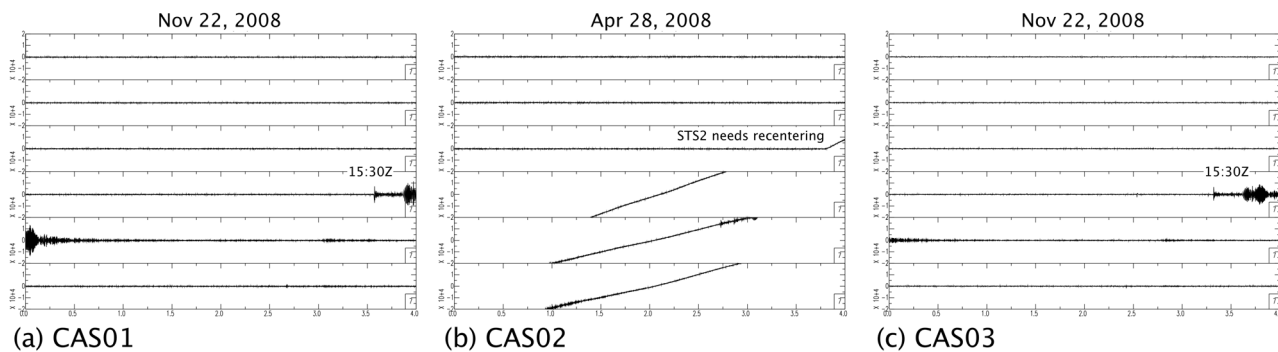
Figure 5. Examples of 2008 data from the prototype stations. Each panel shows one day of data, split into six 4-hour segments. At CAS02 (b), the STS-2 seismometer has drifted too far of center, causing the trend in the data (the mean of each segment is removed from the data before plotting). Panels (a) and (c) show the same event, but given the failure of the GPS units during the first winter (see text) the apparent timing is significantly different between the stations.
