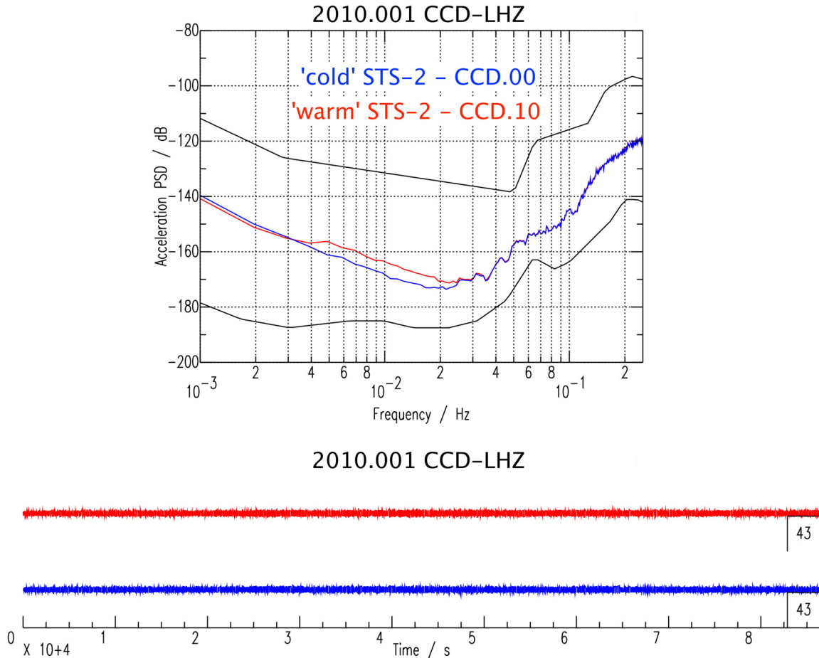
Figure 1. One-day power spectral density plot for CCD station (vertical component, 1sps data) on January 1st, 2010. Also shown are the seismograms for the same day. We run two parallel instruments at Dome-C to ensure redundancy. On January 1st, 2010, these were two STS-2 seismometers, one kept at ambient temperature ( -54^{\circ}\text{C} , blue lines, locid 00) recorded on a Quanterra Q330 digitizer, and one heated to -30^{\circ}\text{C} (red lines, locid 10) recorded on a Quanterra Q4120.
