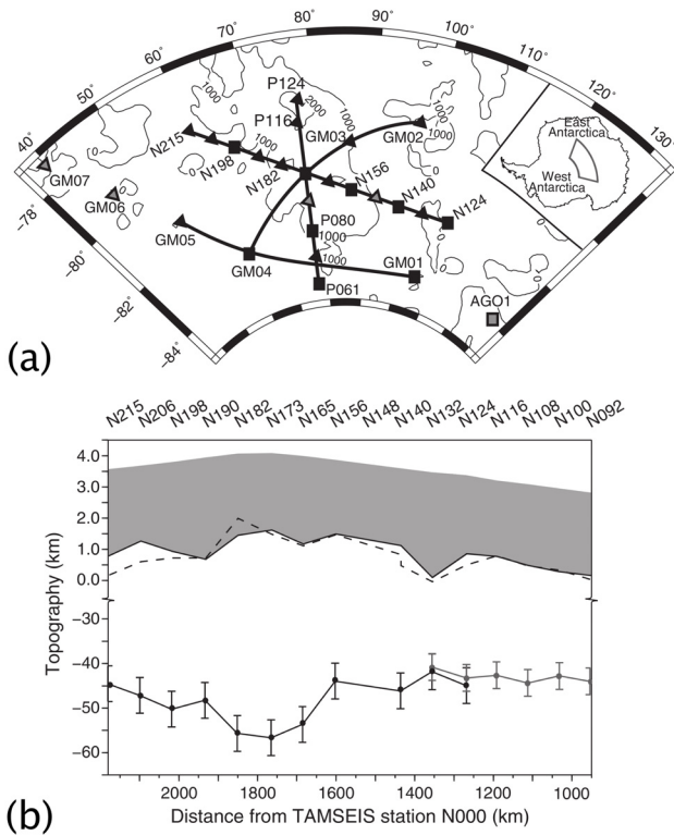
Figure 11. Crustal structure of East Antarctica (after Hansen et al. [2011]). (a) TAMSEIS (N215 to N124), and GAMSEIS stations. (b) Crustal structure derived from joint inversion of S-wave receiver functions and Rayleigh wave dispersion curves.
