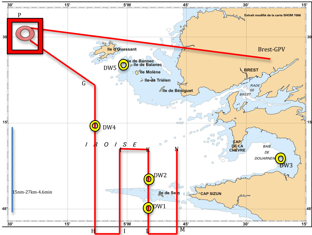
Figure 8. ATR42 Flight plan with KuROS during the PROTEVS campaign. The red pattern has been overflowed three times (once at 2000 m around 12:00 UT , and twice at 3000 m flight level around 13:00 UT and 16:30 UT).
