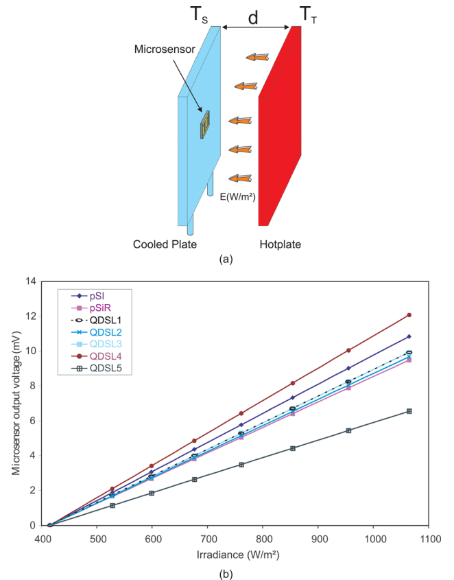
FIG. 4. Characterization of the sensors: (a) Experimental set-up, (b) Experimental output voltages of microsenors with membrane area of 3 \times 3 \text{ mm}^2 versus irradiance E ( \text{W}/\text{m}^2 ).
