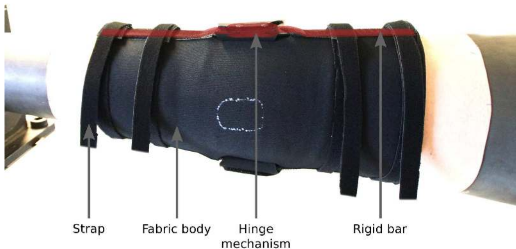
Fig. 3. Medium size generic brace with known geometry and mechanical characteristics.
