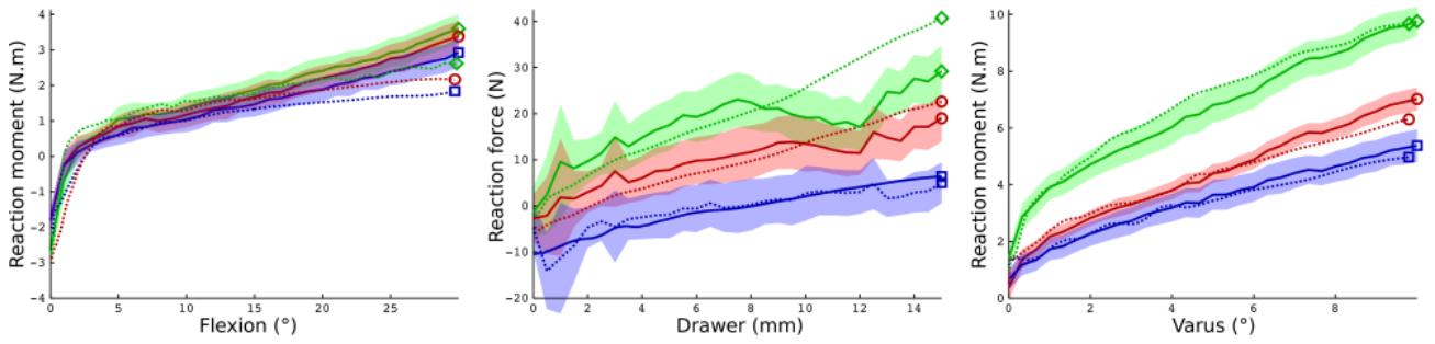
Fig. 6. Comparison of experimental results (solid lines with 90% confidence intervals computed from the Gaussian distribution of 5 repeated tests) and numerical results of the rigid limb model (dotted lines) for three strap tightening levels (blue squares: 0 N; red circles: 30 N; green diamonds: 60 N) for each motion.
