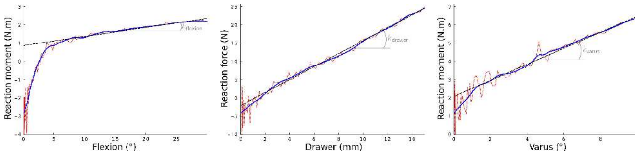
Fig. 5. Typical responses for the different kinematics (flexion, drawer, varus) as obtained by FE simulation of the rigid limb model. In dotted red, the raw response; in solid blue, the response after low-pass filtering; in dashed black, the linear regression line.
