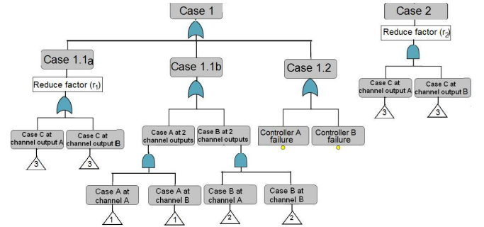
Fig. 4. Fault Tree at system level
