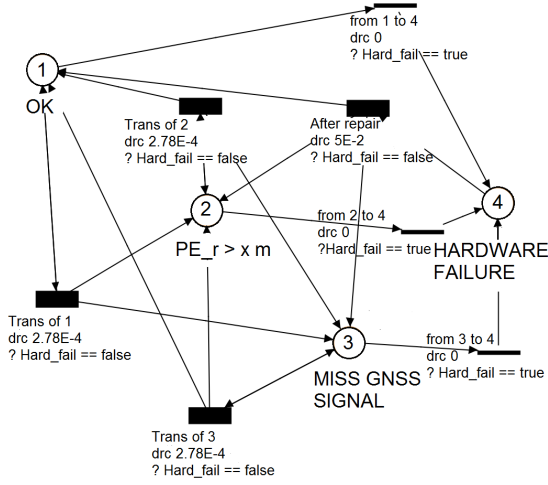
Fig. 7. DSPN structure for position results of GNSS receiver output
