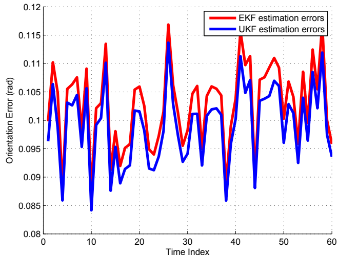
Figure 2: Orientation estimate errors for 100 Monte Carlo trials
