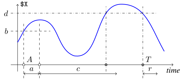
Figure 4. Matching two successive states, the first above level b with a specified duration of a and the second above level d with no duration and within a temporal scope of c . See text for explanations.
