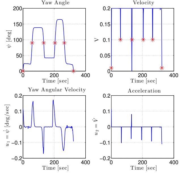
Fig. 4. Time profile of yaw angle \psi , vehicle's velocity and their rate of change \dot{\psi} , \dot{V} respectively
