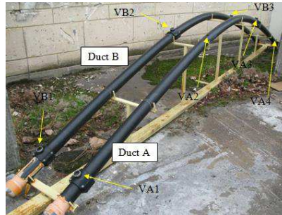
Figure 6: External post stressed duct in Trappes (IFSTTAR laboratoires, France)
