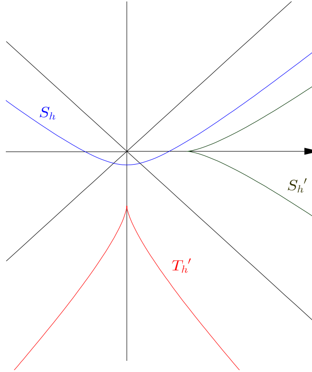
Figure 2. \mathcal{S}_h and its evolute \mathcal{T}_{h'} if h(t) := \cosh(2t)
