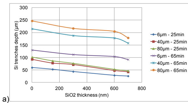
Fig.2: a) Si trenches depth variation versus SiO 2 mask thickness for two Si etching times (25min and 65min) and several trench widths (6µm, 40µm, 80µm). b) Oxide effect on narrowing after photoresist elimination.
