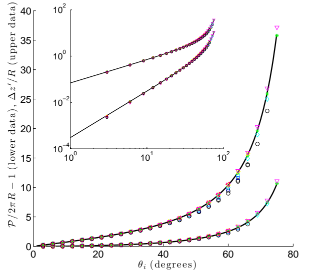
FIG. 5. The relative perimeter (lower data) and the relative distortion (upper data) plotted versus the inclination angle. Solid lines are for the model described in Discussion. Insert: same data plotted on log axes, showing that the agreement is good even at small angles.
