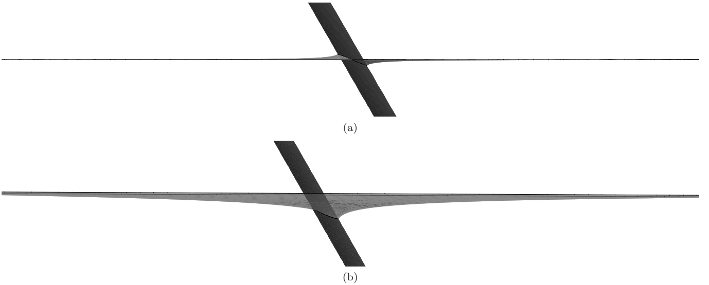
FIG. 1. Side view of a simulation, showing how the interface deforms, in the case \theta_i = 30^\circ , with an imposed contact angle of (a) \theta_w = 90^\circ and (b) \theta_w = 60^\circ .
