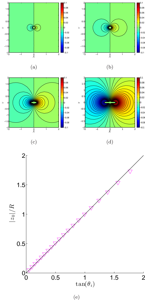
FIG. 8. Film characterization for \theta_w = 90^\circ . Contour plot of film height S for (a) \theta_i = 15^\circ , (b) 30^\circ , (c) 45^\circ and (d) 60^\circ . (e) |z_0|/R versus \tan(\theta_i) for all inclination angles.
