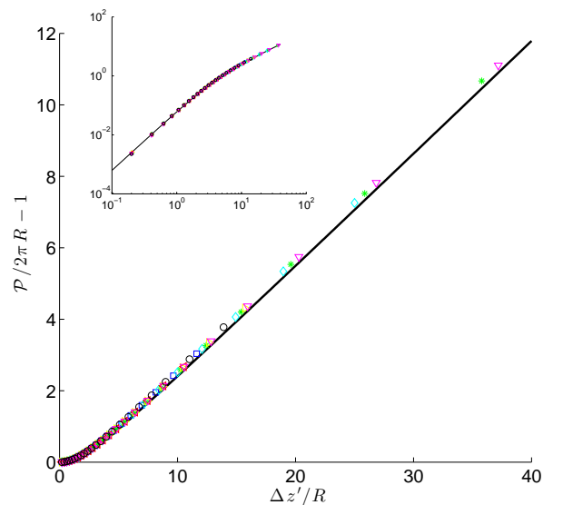
FIG. 9. Ellipse approximation. The dimensionless relative perimeter versus the dimensionless distortion. The solid line holds for the ellipse approximation model described in the main text. Insert: same data plotted on log axes, showing that the agreement is good even at very small \Delta z'/R .
