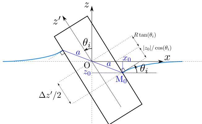
FIG. 7. 2D projection of the film shape for \theta_w = 90^\circ showing the various geometrical quantities defined in the text.
