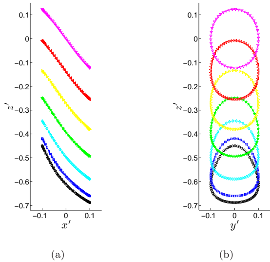
FIG. 3. Projection of the contact line on to (a) the Ox'z' plane and (b) the Oy'z' plane in the reference frame of the cylinder \mathcal{R}' for \theta_i = 30^\circ . The contact angle \theta_w increases upwards, according to the key in Table I.
