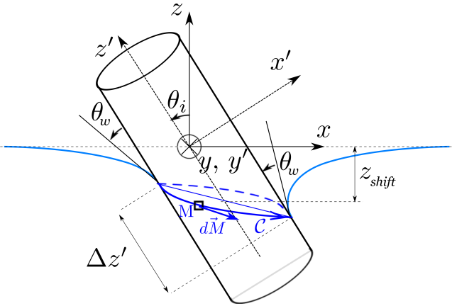
FIG. 2. Schematic representation of the interface-cylinder system.
