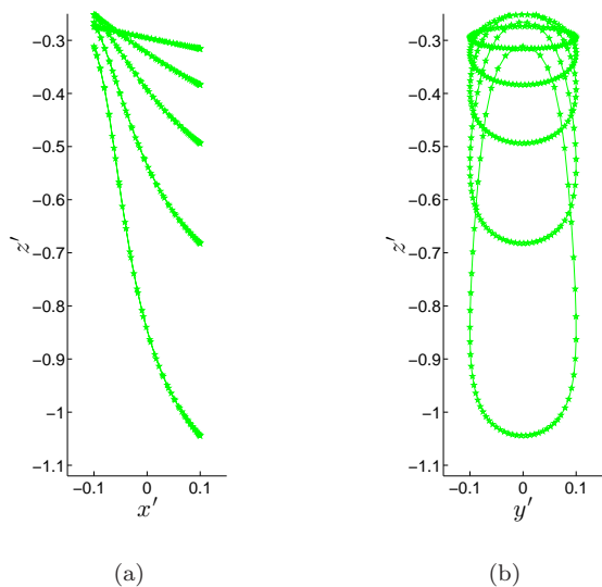
FIG. 4. Projection of the contact line on to (a) the Ox'z' plane and (b) the Oy'z' plane in the reference frame of the cylinder \mathcal{R}' for \theta_w = 45^\circ . From top to bottom \theta_i = 6^\circ, 18^\circ, 30^\circ, 42^\circ and 54^\circ .
