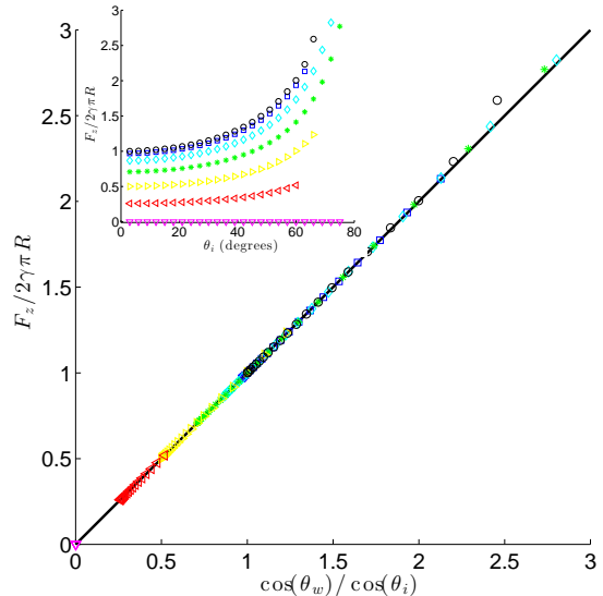
FIG. 6. Force measurements. The dimensionless vertical force F_z/2\pi R versus \cos(\theta_w)/\cos(\theta_i) . One point is slightly off the linear main trend, indicating a lack of mesh refinement when \theta_w \lesssim 10^\circ and \theta_i \gtrsim 65^\circ (see § ). Insert: the dimensionless vertical force vs the inclination angle for all data points.
