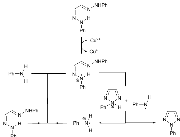
Scheme 2 Mechanism proposed to rationalize the Cu(II)-catalyzed cyclization of glyoxal phenylsazone.
