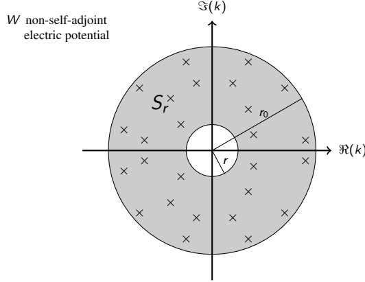
FIGURE 1.1. Complex eigenvalues near a threshold \Lambda_q : For r_0 < \varepsilon sufficiently small, the number of complex eigenvalues \lambda_q(k) = \Lambda_q - k of \mathcal{H} := \mathcal{H}_0 + W in the annulus S_r is bounded by \mathcal{O}\left(\text{Tr}\mathbf{1}_{(r,\infty)}(\rho_q|W|\rho_q)|\ln r|\right) for general potentials W , see Theorem 1.2.
