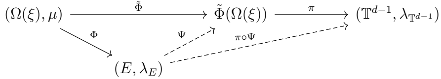
FIGURE 1. Sketch of the maps involved in the proof of Theorem 1: black arrows correspond to continuous maps and dashed arrows to almost everywhere defined maps.
