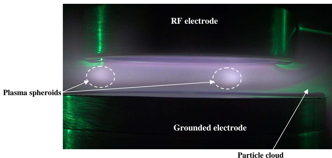
Fig. 1: Plasma spheroids in the discharge. The particle cloud is evidenced in green colour by laser light scattering.
