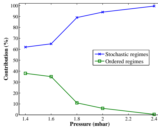
Figure 12. Contribution of the ordered ( \square ) and stochastic ( \times ) regimes as a function of the pressure.
