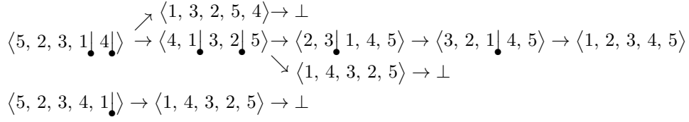
Figure 1: Examples of efficient flips. Sequence \langle 5, 2, 3, 1, 4 \rangle is efficiently sortable (in four flips), but \langle 5, 2, 3, 4, 1 \rangle is not.
