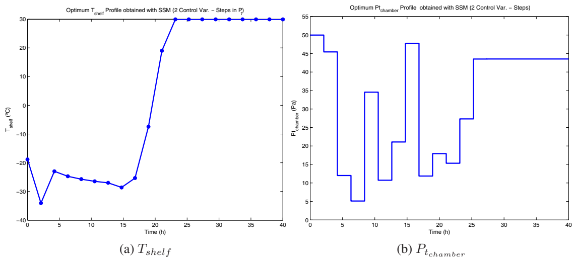
Figure 13: Optimum control profiles obtained with SSm for the dynamic optimization of a freeze-drying cycle. Two control variables case with ramps in T_{shelf} and steps in P_{tchamber} and \rho = 20 .
