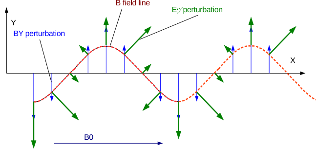
FIGURE 10. Schematic explanation of the parallel electric field E_X parallel to the average magnetic field \vec{B}_0 .
