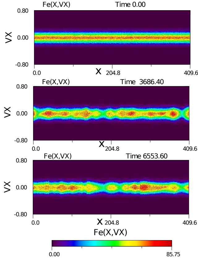
FIGURE 7. AWC009. Snapshots of the electron distribution function as a function of X and of the velocity V_X parallel to the mean magnetic field \vec{B}_0 .
