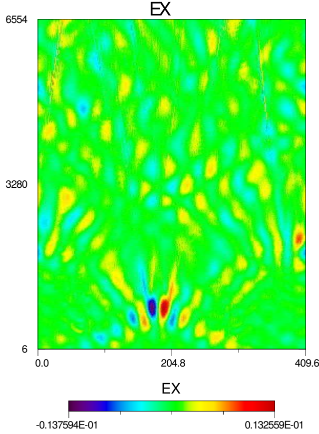
FIGURE 3. AWC009. Temporal stack plot of the electric field E_X(X, t) parallel to \vec{B}_0 . In order to remove plasma oscillations near the plasma frequency, the signal was filtered with a first order low-pass filter (cut-off frequency 0.5\omega_{pe} ).
