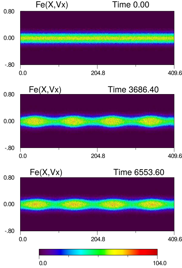
FIGURE 4. AWC008. Snapshots of the electron distribution function as a function of X and the velocity V_x parallel to the local magnetic field \vec{B} .
