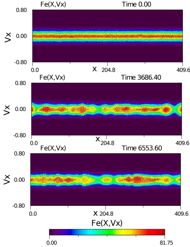
FIGURE 8. AWC009. Snapshots of the electron distribution function as a function of X and the velocity V_x parallel to the local magnetic field \vec{B} .
