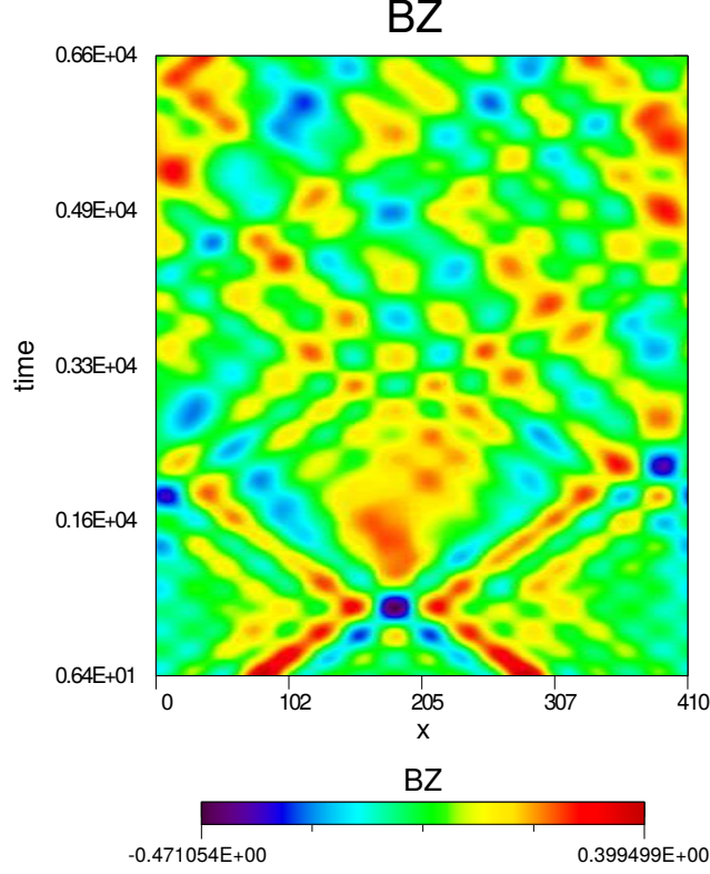
FIGURE 1. AWC009. Temporal stack plot of the transverse magnetic field B_Z(X, t) .
