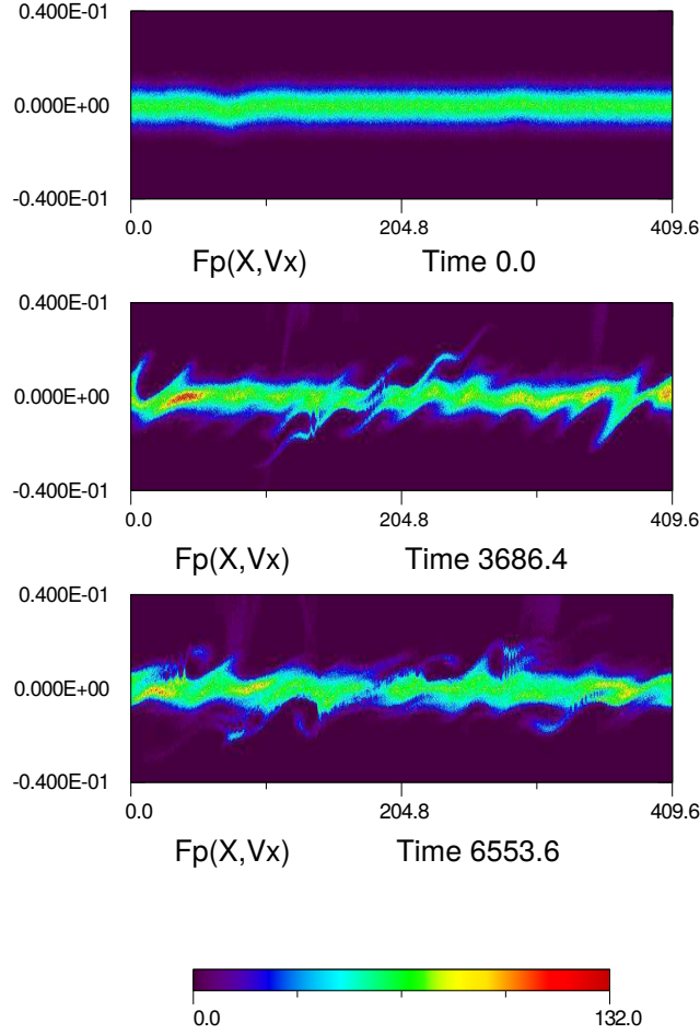
FIGURE 9. AWC009. Snapshots of the ion distribution function as a function of X and the velocity V_x parallel to the local magnetic field \vec{B} .
