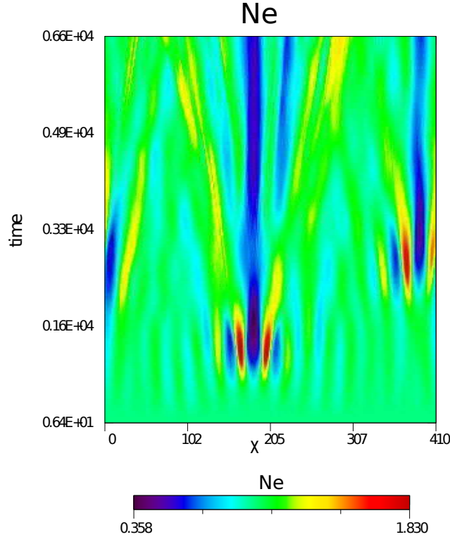
FIGURE 6. AWC009. Temporal stack plot of the electron density N_e(X, t) .
