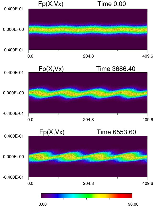
FIGURE 5. AWC008. Snapshots of the ion distribution function as a function of X and the velocity V_x parallel to the local magnetic field \vec{B} .
