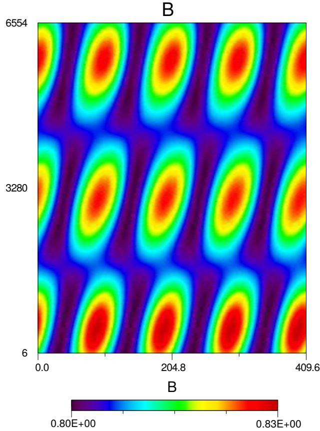
FIGURE 2. AWC008. Temporal stack plot of the magnetic field amplitude B(X, t) .
