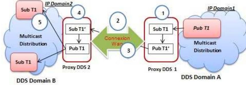
(a) Deployment of Two Proxy DDS Components
