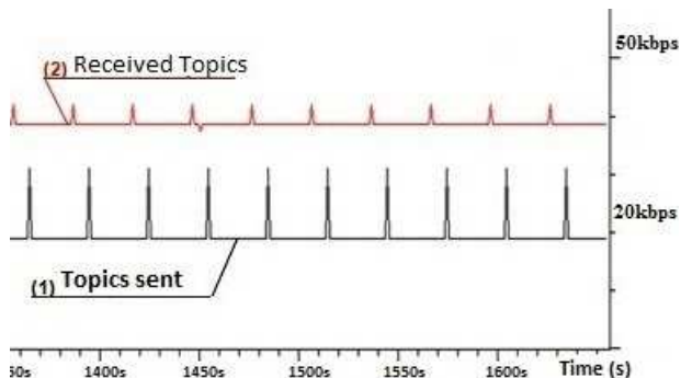
(a) Outgoing Bandwidth Captured on Participant A
