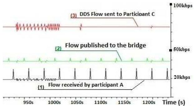
(b) Data Flow with the Topic-Bridge
