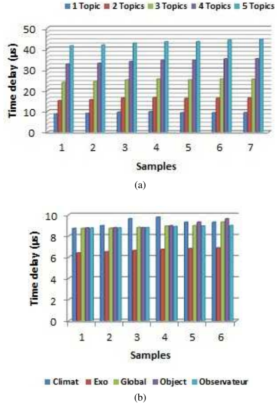
Figure 12: Impact of the number of DDS Topics on the Time Delay for publish/subscribe event
