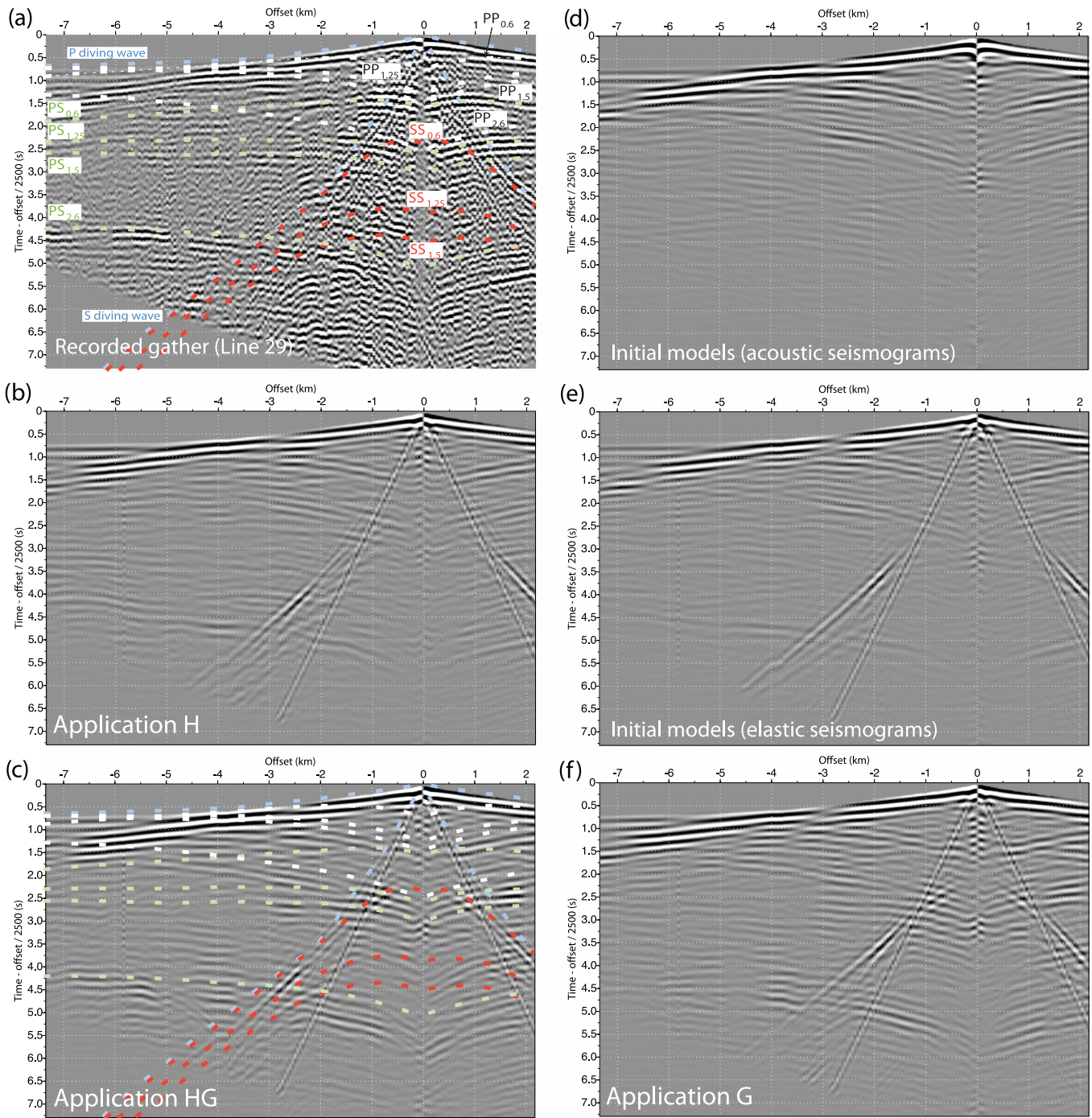
Figure 7. Shot gather recorded by the horizontal geophones of cable 29. The shot was located at X_S = 12.5 km. (a) Recorded data, on which traveltimes of the main converted waves are superimposed, as computed by ray tracing for the final FWI model of application HG . (b, c, f) Synthetic seismograms computed in the final FWI models of applications H (b), HG (c) and G (f). (d, e) Acoustic (d) and elastic (e) synthetic seismograms computed for the initial FWI models (see Fig. 3d, e) (the S -wave velocity model is not taken into account for acoustic modelling). PP_i , PS_i and SS_i denote P – P , P – S and S – S reflection, respectively (propagation in the water layer is not taken into account in the nomenclature), while the index i denotes the depth at which the reflection takes place.
