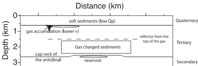
Figure 14. Geological structural scheme of the Valhall field.
