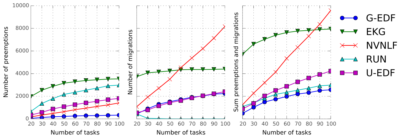
Fig. 4. Number of preemptions and migrations for a system with 8 processors and a (worst-case) total utilization of 95%. The simulation used random durations for the job computation time.
