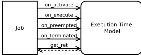
Fig. 3. Interface of any execution time model.
