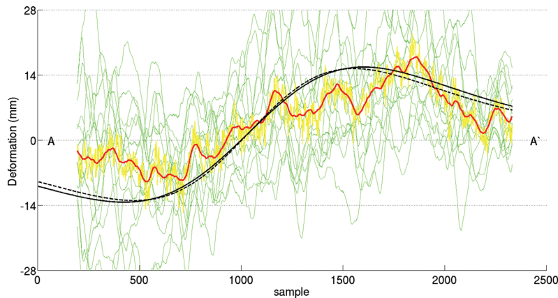
Figure 11. Along cross section A–A4 (see Fig. 10) the line in red shows the ground displacement in the line of sight inferred from the average filtered interferogram. The yellow line is the same quantity but not filtered and the green lines correspond to the single interferograms. The solid black line represents the ground displacement in the line of sight obtained with our model fitting best the GPS data (upper limit of the fault at 17.5 km depth), the dashed line shows the fit when we use a model with the upper limit at 15.5 km depth (corresponding to the lower bound of the blue array at the nominal value of moment tensor in Fig. 8).
