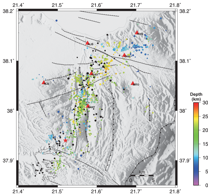
Figure 3. HYPODD relocated aftershocks with colours as a function of depth. Red star indicates main shock epicentre and black dots are the relocated aftershocks occurring the first week (after Galovic et al. 2009).
