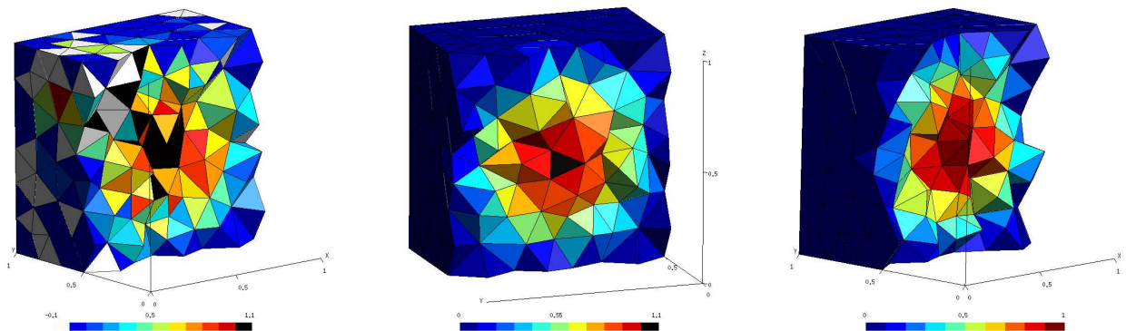
Fig. 3. Maximum principle property for different weights \omega : the adjacent cells have a weight equal to 1.7 (left), the adjacent cells have a weight equal to 2 (middle) while the right panel displays the approximation for \omega = 4 (very close to the exact solution). White cells correspond to negative values while black cells correspond to values larger than one.
