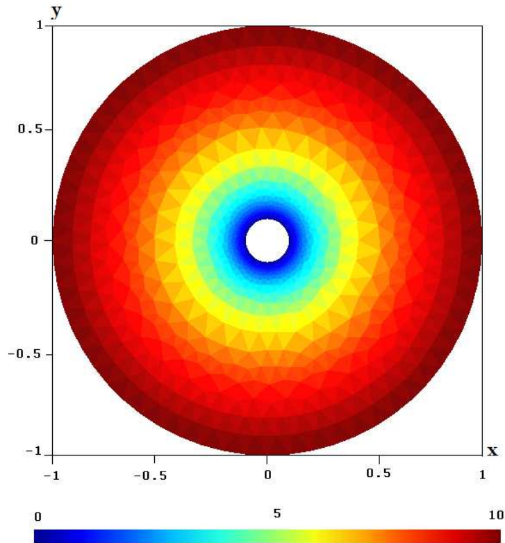
Fig. 6. Solution of the Poisson equation for the annulus problem.
