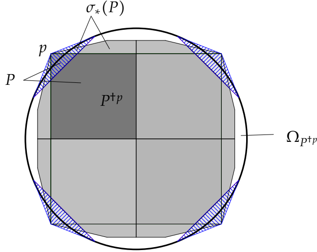
FIGURE 11. The starting of the tiling given here is obtained thanks to a square with three right angles and one loxodromic vertex: p . The convex set \Omega_P is the union of the convex set \Omega_{P^+} and the \Gamma_P -orbits of the hatching zone. The limit set is the boundary of \Omega_{P^+} minus the interior of the \Gamma_P -orbits of the hatching zone.
