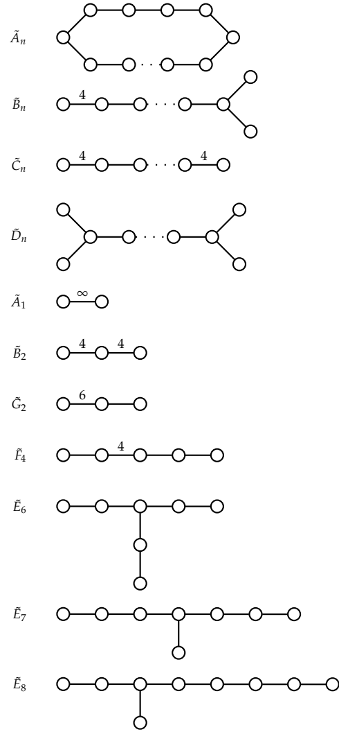
FIGURE 3. Irreducible affine diagram
