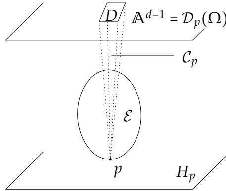
FIGURE 8. Action of a parabolic subgroup
