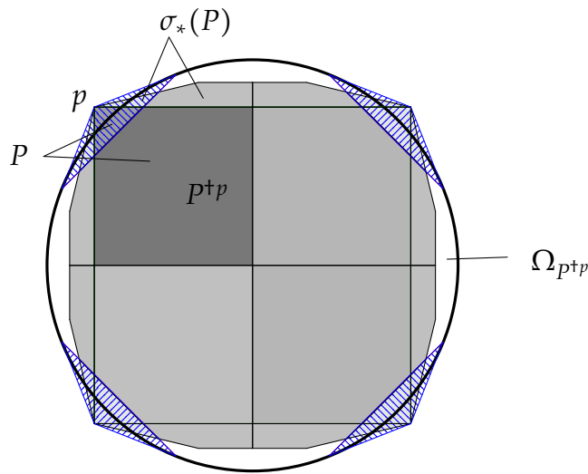
FIGURE 11. The starting of tiling given here is obtained thanks to a square with three right angle and one loxodromic vertex: p . The convex \Omega_P is the union of the convex \Omega_{P^+p} and the \Gamma_P -orbits of the hatching zone. The limit set is the boundary of \Omega_{P^+p} minus the interior of the \Gamma_P -orbits of the hatching zone.
