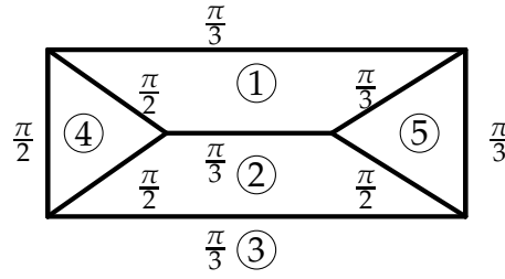
FIGURE 13. An indecomposable quasi-divisible prism which gives a non-strictly convex convex
