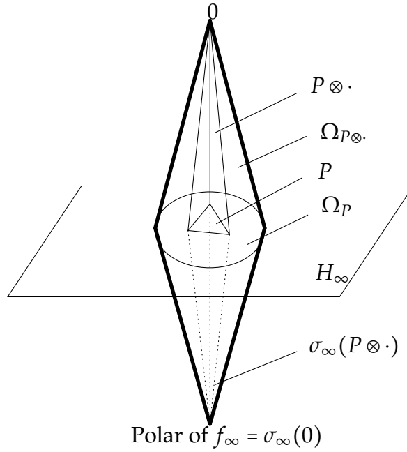
FIGURE 6. The Coxeter cone above a Coxeter polytope
