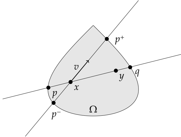
FIGURE 1. Hilbert distance
