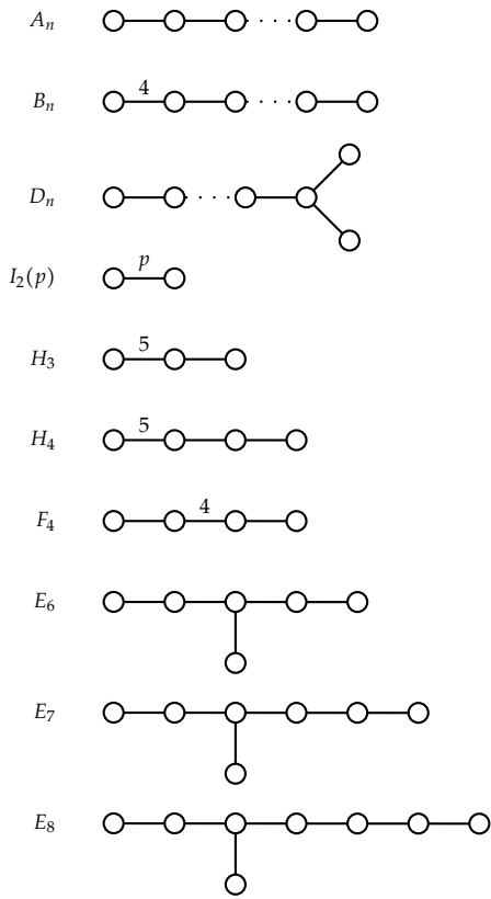
FIGURE 2. Irreducible spherical diagram
