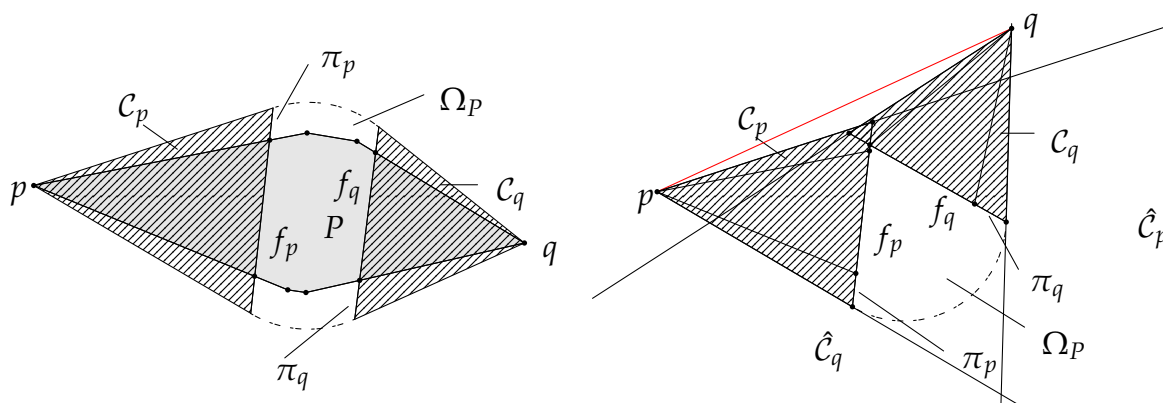
FIGURE 10. A possible situation and an impossible situation
