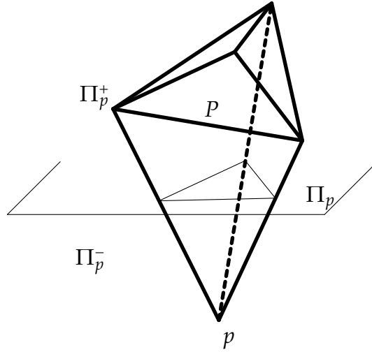
FIGURE 9. Illustration of Truncability of p
