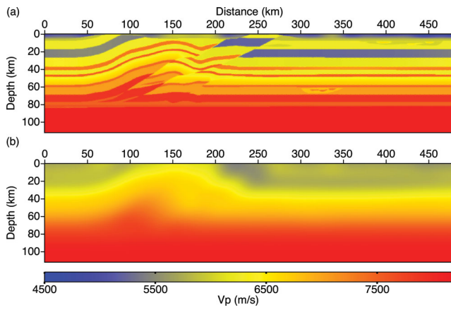
Figure 6. Lithospheric SEG/EAGE overthrust model (a) True and (b) starting P -wave velocity models. The S -wave velocity model is derived from the P -wave velocity model using a constant Poisson ratio of 0.25.
