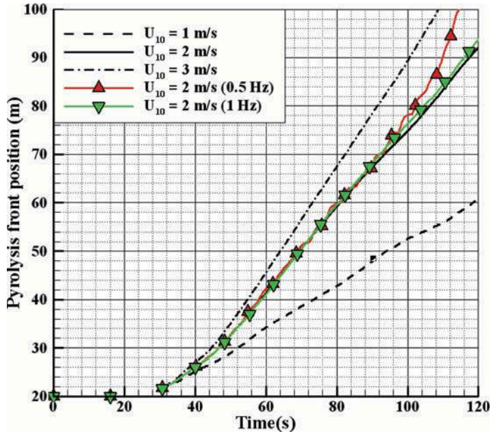
Figure 10 Time evolution of pyrolysis front ( T_S = 500 K) calculated for various wind conditions (steady: U_{10} = 1, 2, and 3 m/s; unsteady: \langle U_{10} \rangle = 2 m/s, \langle \Delta U_{10} \rangle = 1 m/s, ( F = 0.5 and 1 Hz)).
