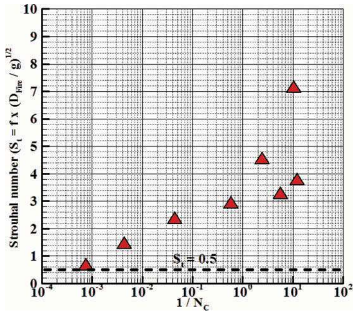
Figure 7 Evolution of the buoyant Strouhal number (plume scales) as a function of the convective Byram number.
