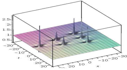
Figure 1: Solution to NLS, N=3 , \tilde{a}_1 = 10^4 : triangle with 6 peaks; on the right, N=4 , \tilde{a}_1 = 10^3 : triangle with 10 peaks.
