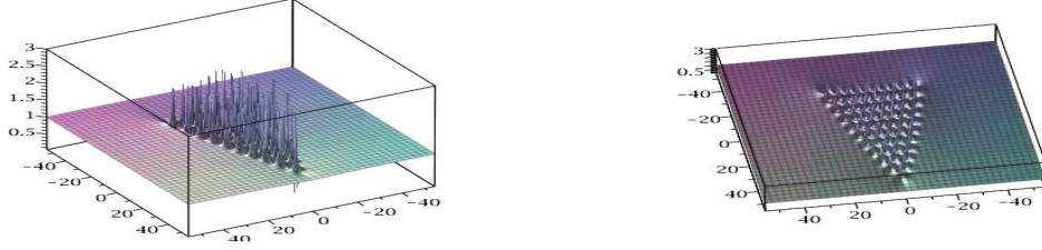
Figure 6: Solution to NLS, N=10 , \tilde{a}_1 = 10^3 : triangle with 55 peaks; on the right, sight of top.
