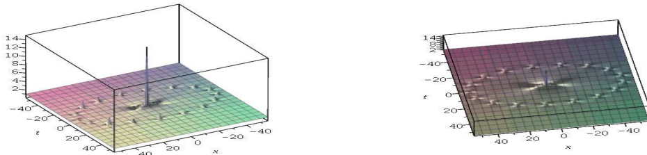
Figure 11: Solution to NLS, N=9 , \tilde{a}_8 = 10^{20} : ring with 17 peaks, P_7 in the center; on the right, sight of top.
