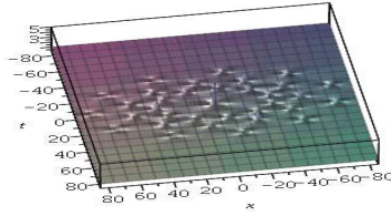
Figure 19: Solution to NLS, N=8 , \tilde{a}_5 = 10^{20} : 3 rings with 11 peaks, P_2 in the center; on the right, sight of top.
