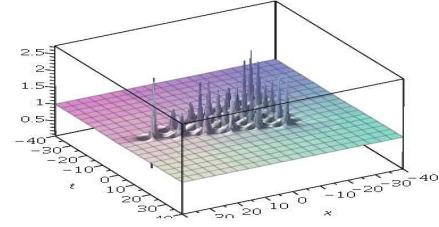
Figure 2: Solution to NLS, N=5 , \tilde{a}_1 = 10^4 : triangle with 15 peaks; on the right, N=6 , \tilde{a}_1 = 10^3 : triangle with 21 peaks.
