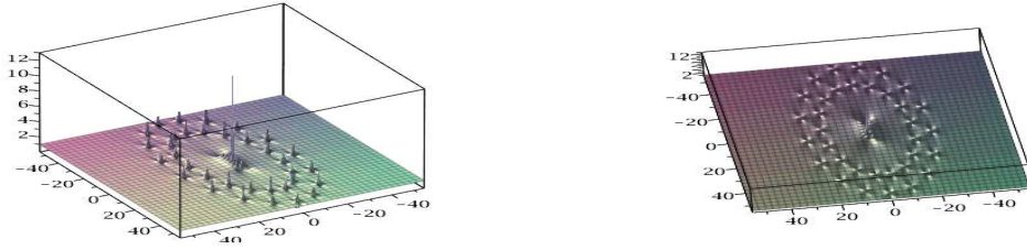
Figure 17: Solution to NLS, N=10 , \tilde{a}_8 = 10^{19} : 2 rings with 17 peaks, P_6 in the center; on the right, sight of top.
