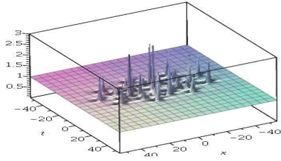
Figure 18: Solution to NLS, N=7 , \tilde{a}_4 = 10^{10} : 3 rings with 9 peaks, P_1 in the center; on the right, sight of top.
