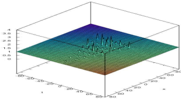
Figure 4: Solution to NLS, N=8 , \tilde{a}_1 = 10^6 : triangle with 36 peaks; on the right, sight of top.
