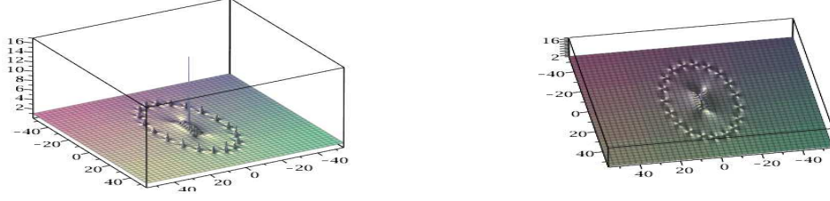
Figure 12: Solution to NLS, N=10 , \tilde{a}_9 = 10^{19} : ring with 19 peaks, P_8 in the center; on the right, sight of top.
