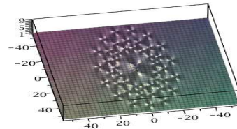
Figure 21: Solution to NLS, N=10 , \tilde{a}_7 = 10^{16} : 3 rings with 15 peaks, P_4 in the center; on the right, sight of top.
