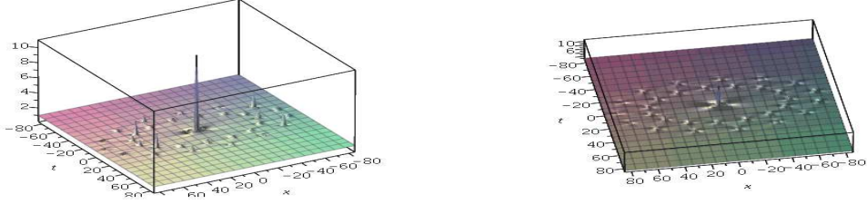
Figure 16: Solution to NLS, N=9 , \tilde{a}_7 = 10^{20} : 2 rings with 15 peaks, P_5 in the center; on the right, sight of top.
