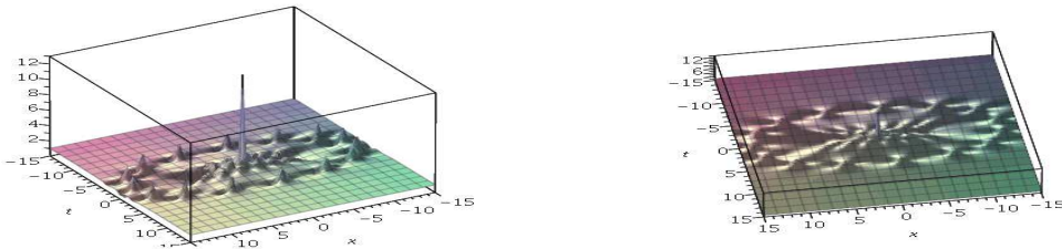
Figure 10: Solution to NLS, N=8 , \tilde{a}_7 = 10^{10} : ring with 15 peaks, P_6 in the center; on the right, sight of top.
