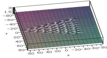
Figure 3: Solution to NLS, N=7 , \tilde{a}_1 = 10^4 : triangle with 28 peaks; on the right, sight of top.
