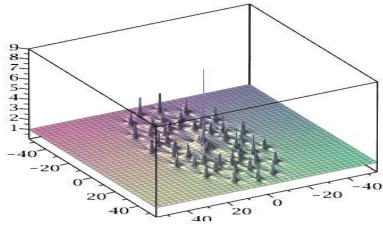
Figure 21: Solution to NLS, N=10 , \tilde{a}_7 = 10^{16} : 3 rings with 15 peaks, P_4 in the center; on the right, sight of top.
