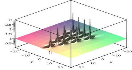
Figure 1: Solution to NLS, N=3 , \tilde{a}_1 = 10^4 : triangle with 6 peaks; on the right, N=4 , \tilde{a}_1 = 10^3 : triangle with 10 peaks.
