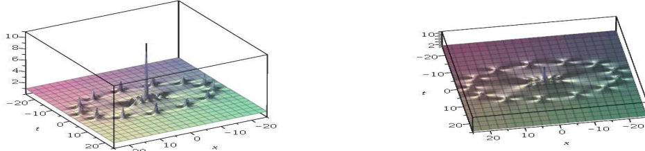
Figure 9: Solution to NLS, N=7 , \tilde{a}_6 = 10^{12} : ring with 13 peaks, P_5 in the center; on the right, sight of top.
