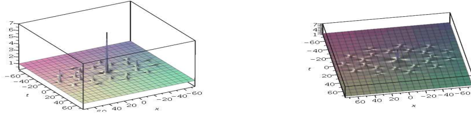
Figure 14: Solution to NLS, N=7 , \tilde{a}_5 = 10^{15} : 2 rings with 11 peaks, P_3 in the center; on the right, sight of top.
