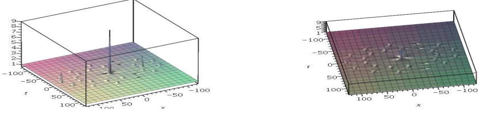
Figure 15: Solution to NLS, N=8 , \tilde{a}_6 = 10^{20} : 2 rings with 13 peaks, P_4 in the center; on the right, sight of top.
