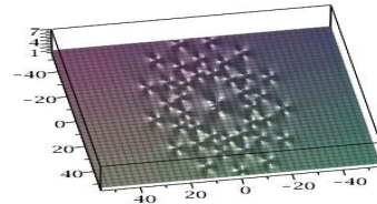
Figure 20: Solution to NLS, N=9 , \tilde{a}_6 = 10^{15} : 3 rings with 13 peaks, P_3 in the center; on the right, sight of top.
