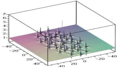
Figure 20: Solution to NLS, N=9 , \tilde{a}_6 = 10^{15} : 3 rings with 13 peaks, P_3 in the center; on the right, sight of top.
