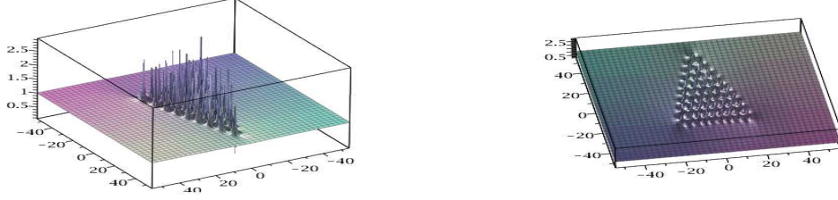
Figure 5: Solution to NLS, N=9 , \tilde{a}_1 = 10^3 : triangle with 45 peaks; on the right, sight of top.
