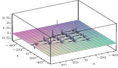
Figure 2: Solution to NLS, N=5 , \tilde{a}_1 = 10^4 : triangle with 15 peaks; on the right, N=6 , \tilde{a}_1 = 10^3 : triangle with 21 peaks.
