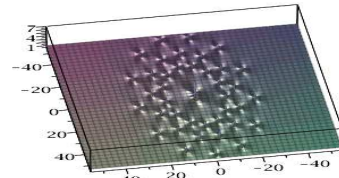
Figure 20: Solution to NLS, N=9 , \tilde{a}_6 = 10^{15} : 3 rings with 13 peaks, P_3 in the center; on the right, sight of top.
