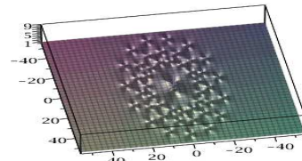
Figure 21: Solution to NLS, N=10 , \tilde{a}_7 = 10^{16} : 3 rings with 15 peaks, P_4 in the center; on the right, sight of top.
