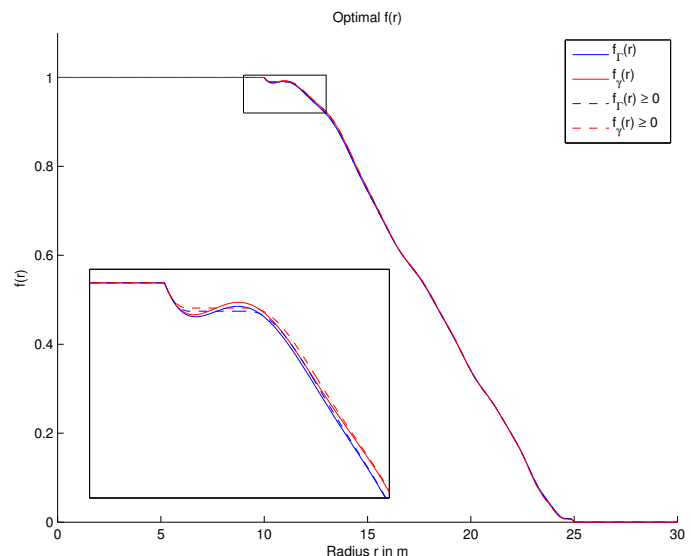
Fig. 3. Radial cut of the attenuation of the functions f(r) for aperture and focal optimization at a wavelength of 562 nm. The dashed curves denoted as \geq 0 correspond to an optimization with \alpha \geq 0 constraint.
