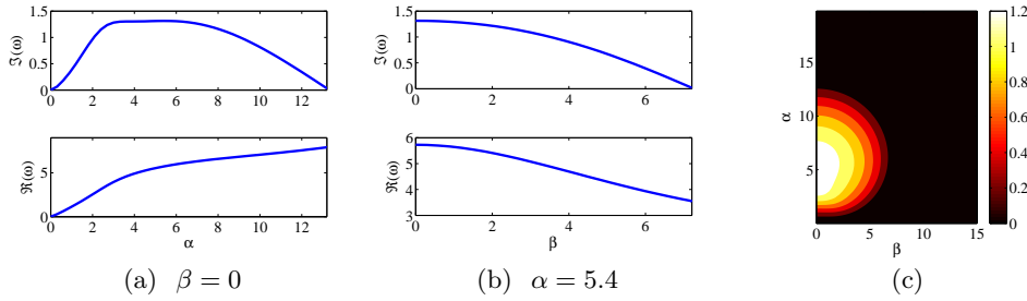
FIGURE 6. The same as Figure 5, but with (m, Re, S) = (30, 100, 0.1) .
