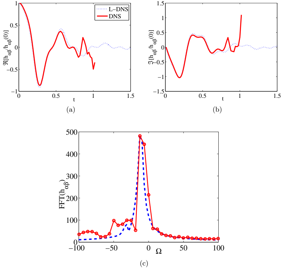
FIGURE 10. Dynamics of the spanwise Fourier mode \alpha = (\alpha_0, \beta_0) . (a) Real part of h_\alpha(t)/h_\alpha(0) with a comparison between the full DNS and the linearized DNS; (b) imaginary part of the same; (c) Spectral analysis (frequency space) based on the linearized DNS (broken line) and the full nonlinear DNS (solid line, with dots, spectrum taken between t = 0 and t = 1.02 ). The two most-prominent peaks in the L-DNS in fact coincide with the OSS modal frequencies.
