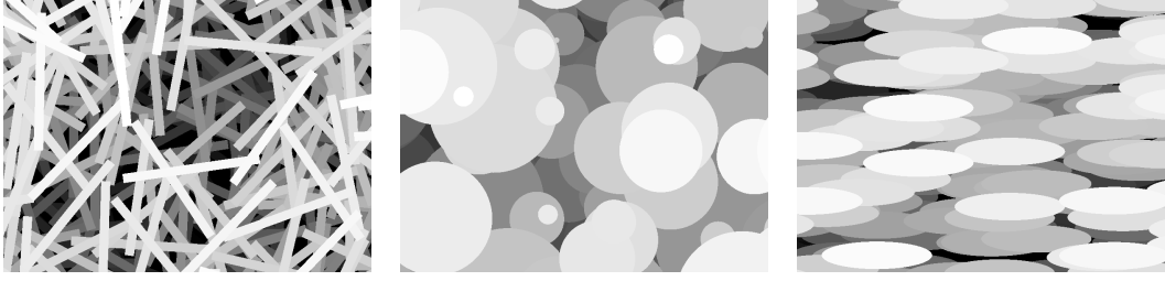
Figure 4: Realizations of three different Boolean random fields with uniformly distributed gray-levels. The grain distributions are the ones presented in Fig. 1.
