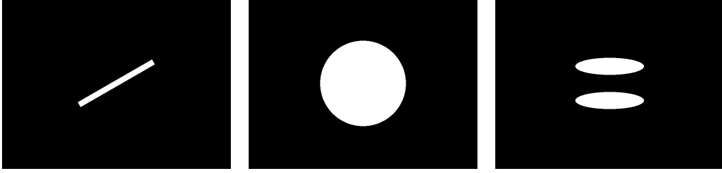
Figure 1: Representation of the three grain distributions used for the simulations of shot noise models, Boolean models, colored dead leaves models, and transparent dead leaves models. (see Fig. 2, Fig. 3, Fig. 4, Fig. 5, and Fig. 6). Left: a rectangle randomly oriented according to a uniform distribution over [0, \pi] ; Middle: a disc having a radius uniformly distributed over an interval [0, r_{\max}] (the displayed disc has size r_{\max} ); Right: a fixed non convex set constituted of two disjoint ellipses.
