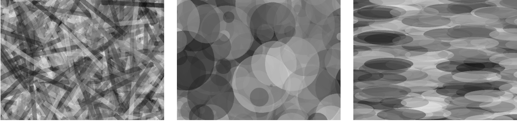
Figure 6: Realizations of three different transparent dead leaves r.f. with uniformly distributed gray-levels and transparency coefficient \alpha = 0.4 . The grain distributions are the ones presented in Fig. 1.
