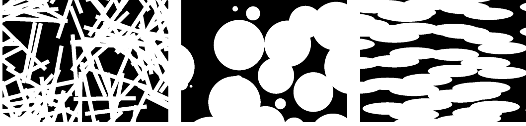
Figure 3: Realizations of three different Boolean random sets for which the grain distributions are the ones presented in Fig. 1.
