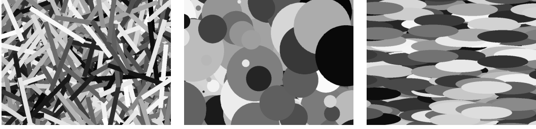
Figure 5: Realizations of three different colored dead leaves r.f. with uniformly distributed gray-levels. The grain distributions are the ones presented in Fig. 1.
