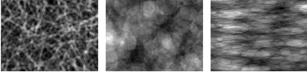
Figure 2: Realizations of three different Poisson shot noises with uniformly distributed gray-levels. The grain distributions are the ones presented in Fig. 1.
