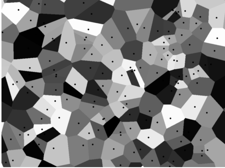
Figure 7: A realization of a colored Poisson-Voronoi tessellation with uniformly distributed gray levels. The points of the underlying Poisson point process are displayed in black.
