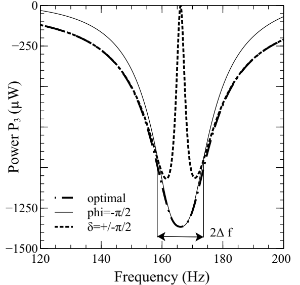
Figure 17: Electric power P_3 for \Gamma = 10m/sec^2 , as a function of the frequency f = \frac{\omega}{2\pi} ; \bullet optimal operating conditions; --- optimal mechanical power strategy; --- Lower voltage strategy.
