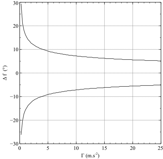
Figure 18: \Delta f as a function of \Gamma for the prototype; simulation results.
