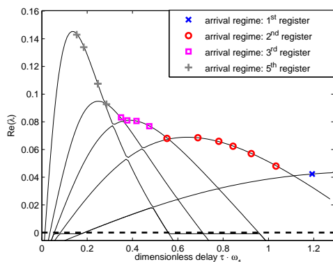
Figure 8: Lines: real parts of roots \kappa (linearised model), as function of \tilde{\tau} , for the G_4 fingering. Markers: time-domain simulation of steps of P_{mouth} with rise time of 40ms ; representation of the arrival register as function of the value \tilde{\tau}_c corresponding to the step amplitude P_t .
