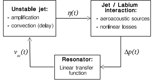
Figure 2: Basic modeling of sound production mechanism in flute-like instruments, as a feedback loop system [1].
