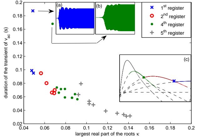
Figure 7: Time-domain simulation of mouth pressure steps, for the A_4 fingering. Transient duration of v_{ac} with respect to the largest value \Re(\kappa) at the value of \tilde{\tau}_c corresponding to the amplitude P_t of the step. (a) and (b): temporal signal v_{ac} with respect to time for the two pathological points. (c): \Re(\kappa) of the linearised model, with respect to \tilde{\tau} .
